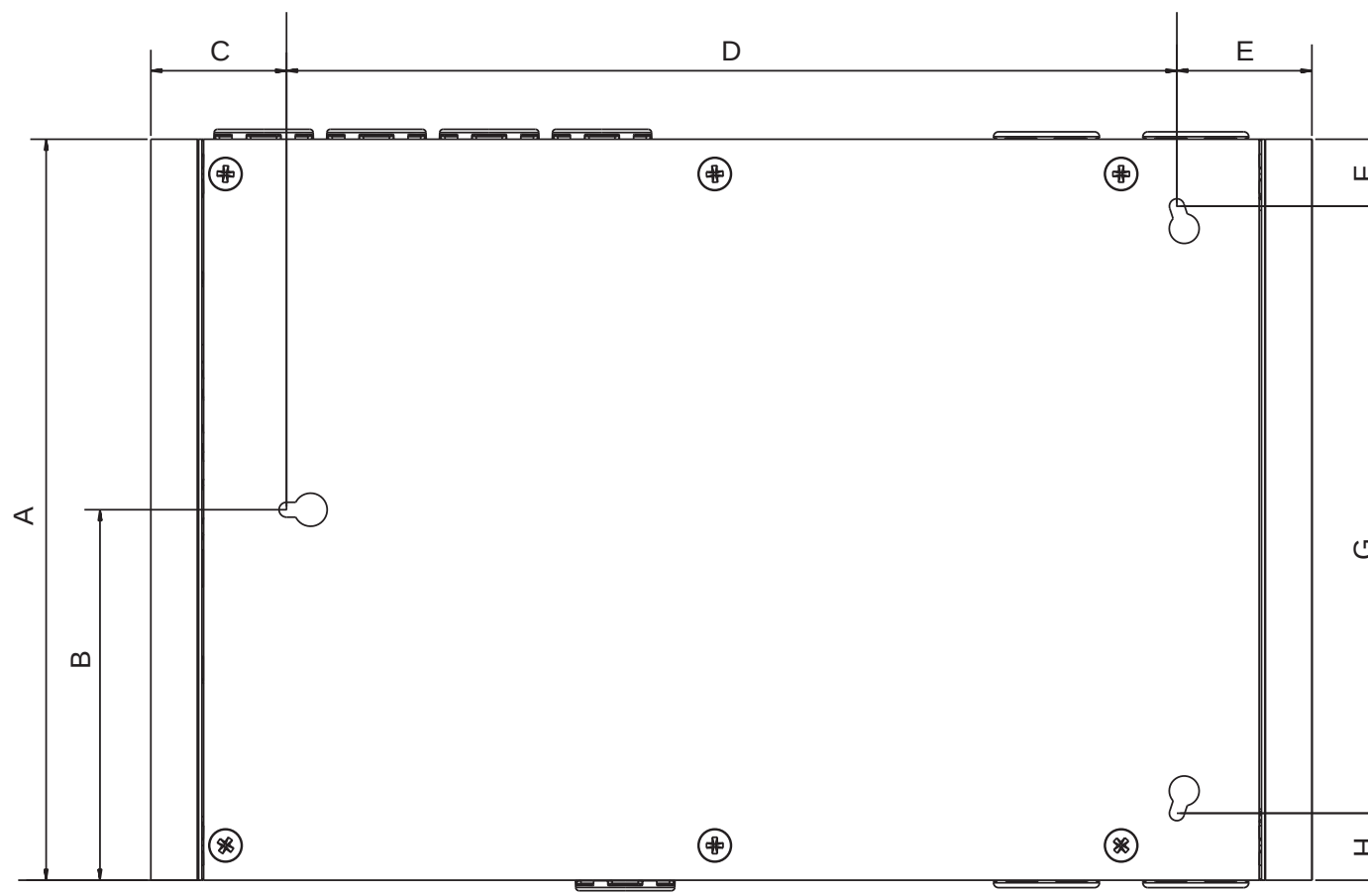
Figure 2-11: Rear Dimensions with hole locations for direct mounting
