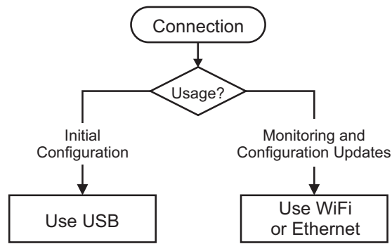
Figure 2-8: Connection Method
