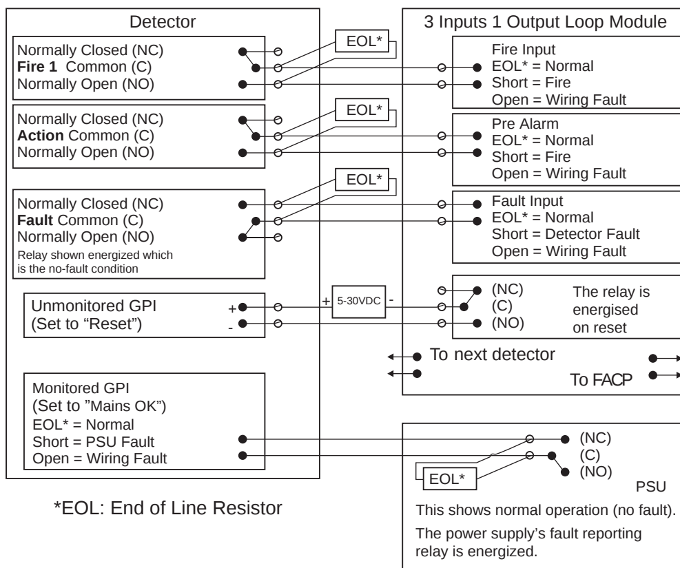
Figure 4-38: Input/Output Loop Module with EOL
