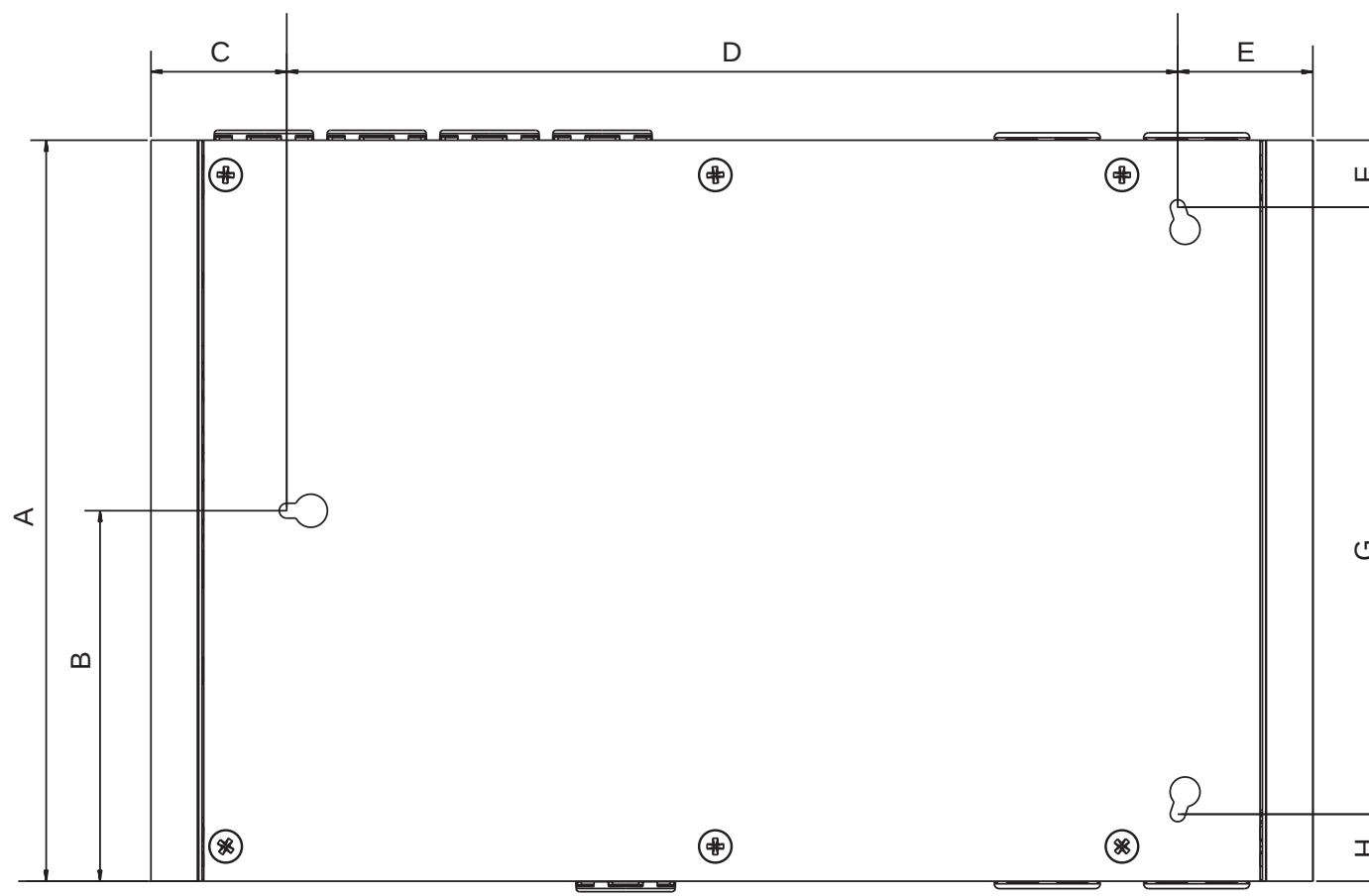
Figure 2-6: Rear Dimensions with hole locations for direct mounting
