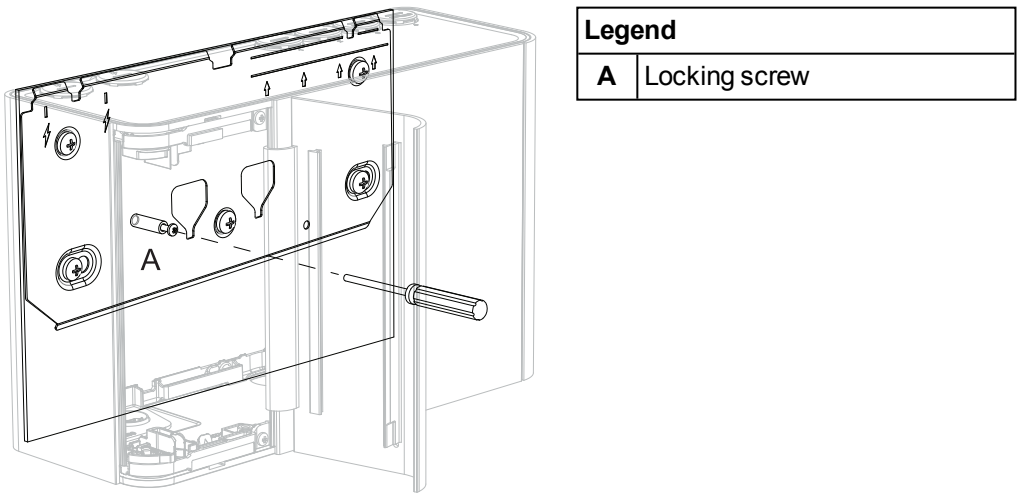
Figure 4-22: Locking Screw
