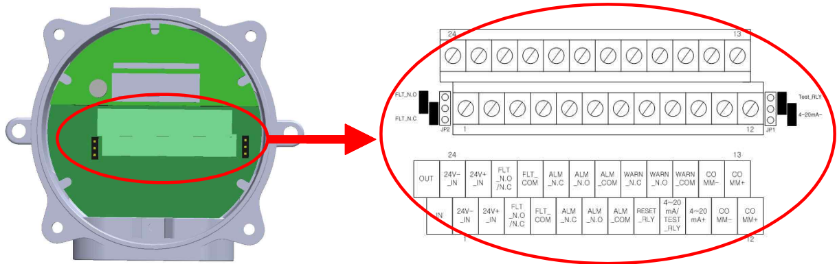
[Figure 2] TB1 Terminal address at product cover
