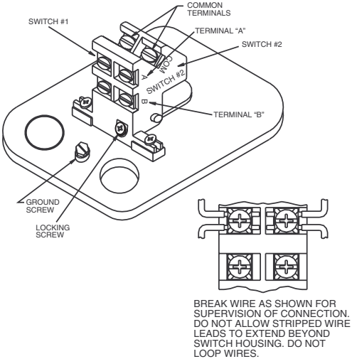
FIGURE 3. SWITCH TERMINALS:
