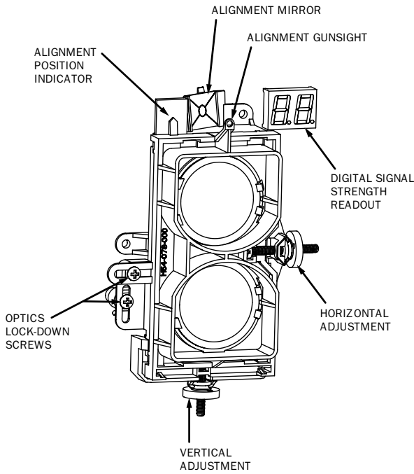
Figure 12. Coarse Alignment Procedure
