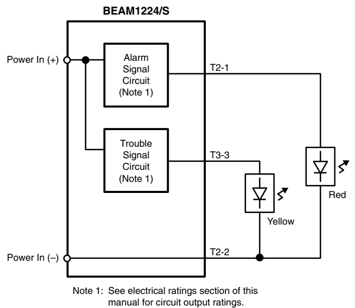
Figure 9. Wiring Diagram (RTS451)
