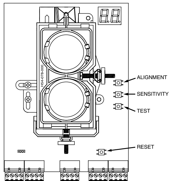
Figure 10. Switch Locations
