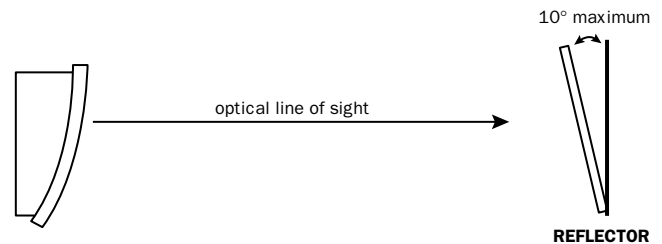
Figure 5b. Reflector Mounting Guidelines
