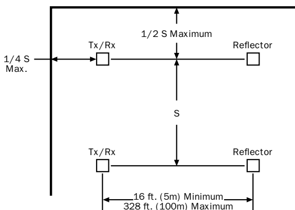
Figure 2. Spacing for smooth ceiling (top view):
