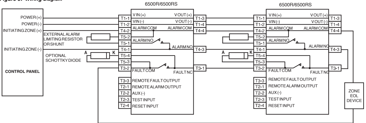
Figure 5: Wiring Diagram
