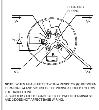
Figure 1: Base Terminal Wiring
