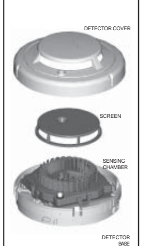
Figure 3: 2351E Optical Smoke Detector
