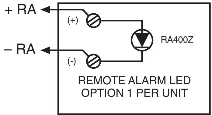
FIGURE 8. WIRING DIAGRAM FOR DNR TO RA400Z:
