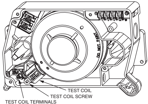
FIGURE 8. DNR WITH OPTIONAL TEST COIL
