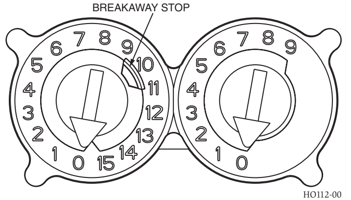
FIGURE 7. ROTARY ADDRESS SWITCHES
