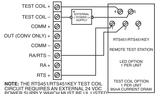
FIGURE 9. WIRING DIAGRAM FROM DNR TO RTS451/RTS451KEY:
