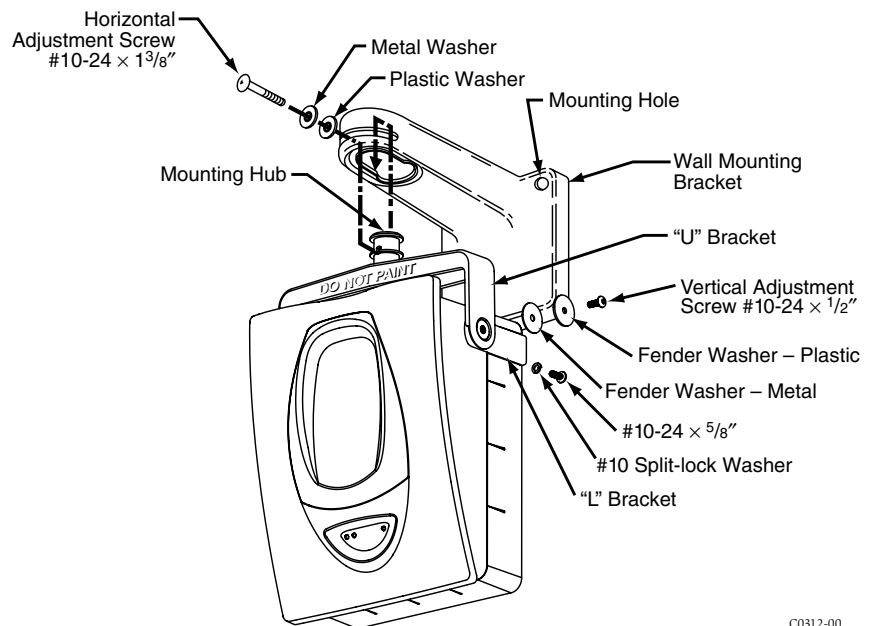
Figure 3. Wall mounting transmitter/receiver unit:
