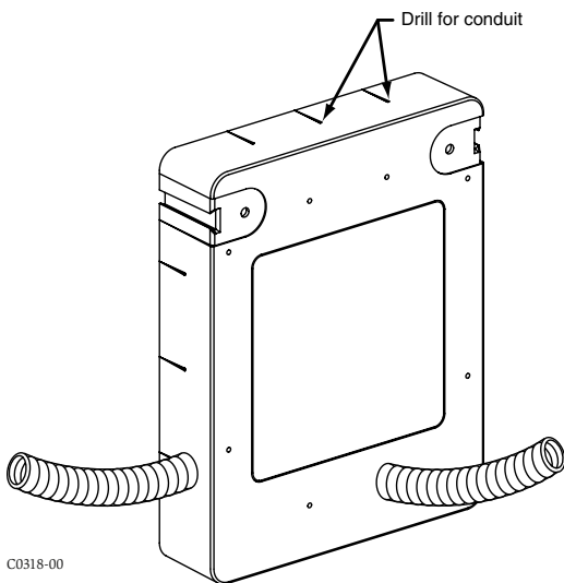
Figure 2. BEAMSMK wiring locations:
