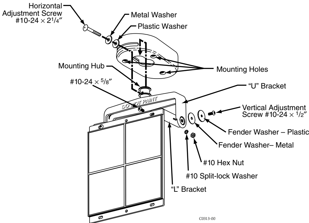
Figure 4. Ceiling mounting reflector:
