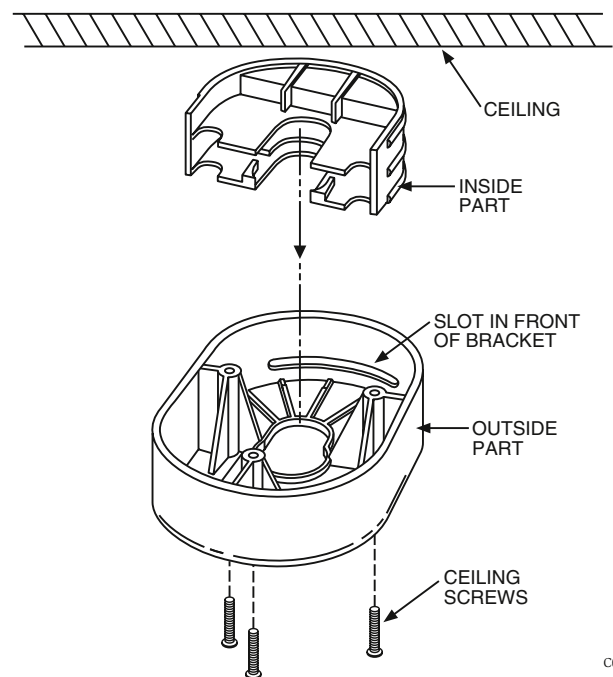
Figure 1. Ceiling mount bracket assembly:
