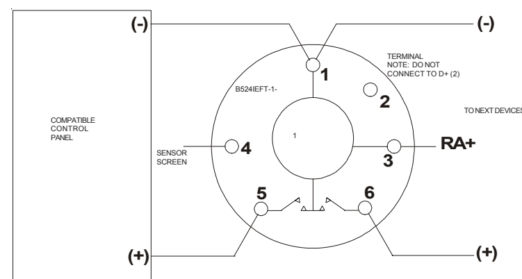
Figure 3. Typical Wiring Diagram
