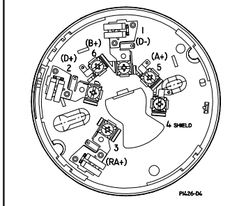
Figure 1: Terminal Layout
