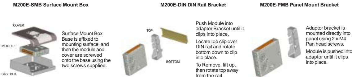
FIGURE 1: MODULE MOUNTING METHODS
